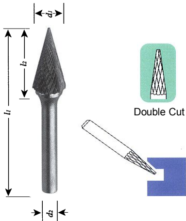
14° & 25° Cone Shape (M Series)
