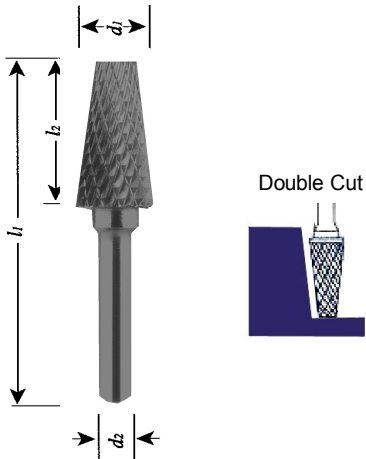
Flat End Taper (S Series)
